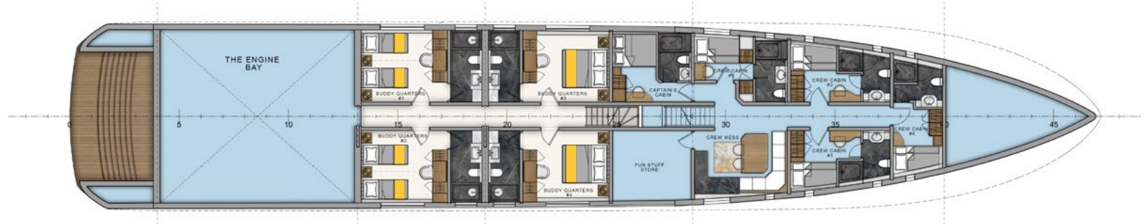
LOWER DECK
