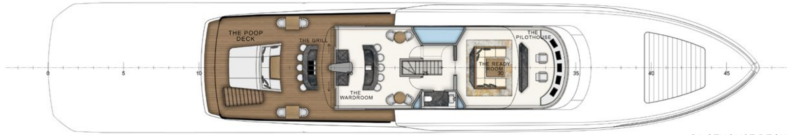
PILOTHOUSE DECK
