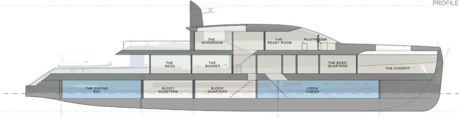
SECTION
