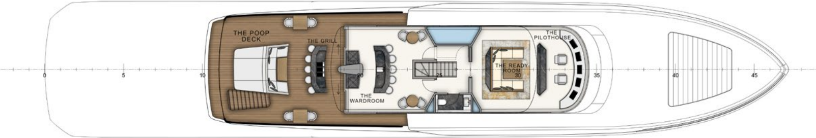
PILOTHOUSE DECK
